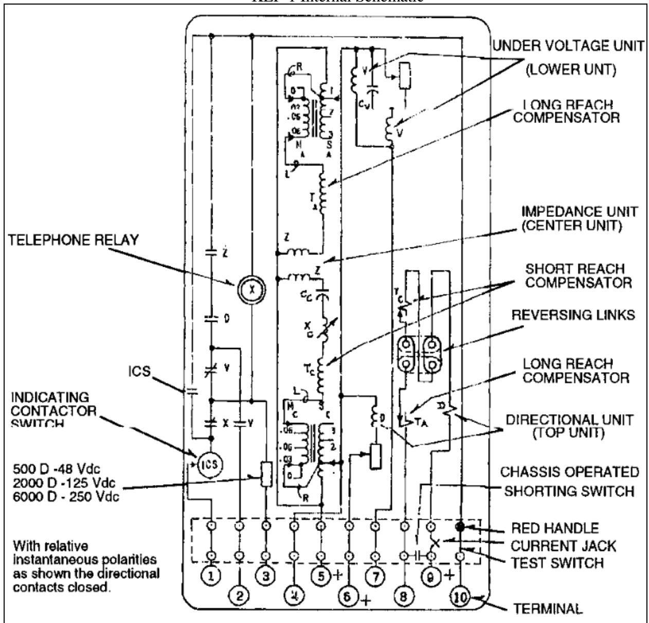
KLF-1 Internal Schematic
