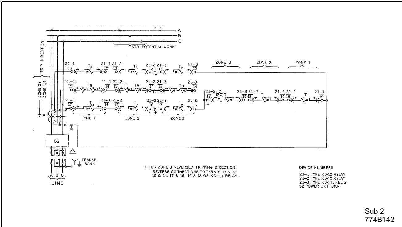
Figure 22: External Schematic: Two Type KD-10 Relays, One KD-11 Relay, Wye-Delta Bank Termination with Delta on Relay Side
