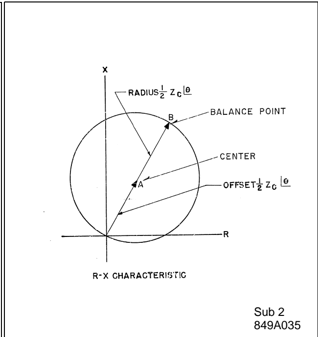
Figure 11: Impedance Circle for Three-Phase Unit in the Type KD-10 Relay
