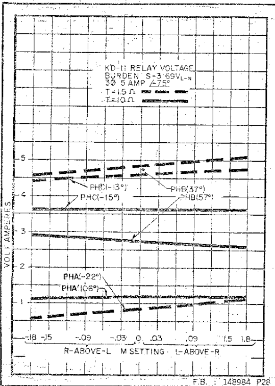
Figure 18b: Type KD-11 Burden Curves
