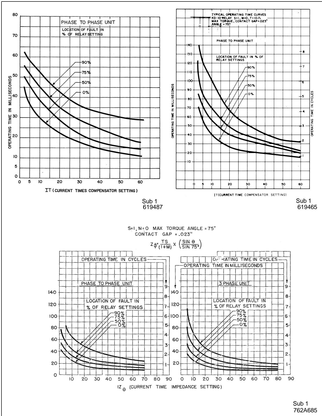
Figure 14: Typical Operating Time Curves Normal Voltages Before Fault 120 Volts, Phase-to-Phase Unit
