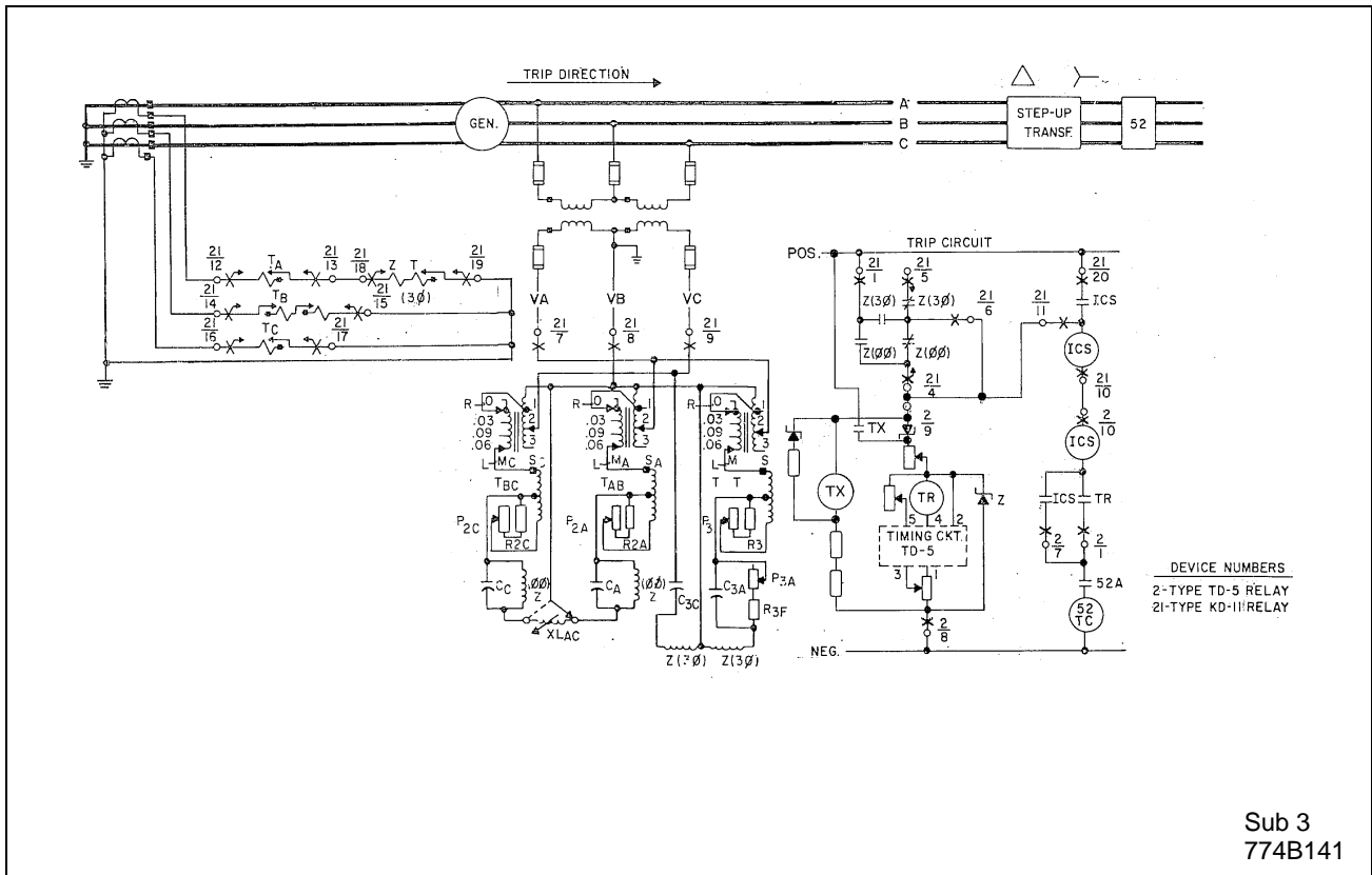
Figure 23: External Schematic: Type KD-11 Relay with Type TD-5 Timing Relay for Generator Back Up Protection
