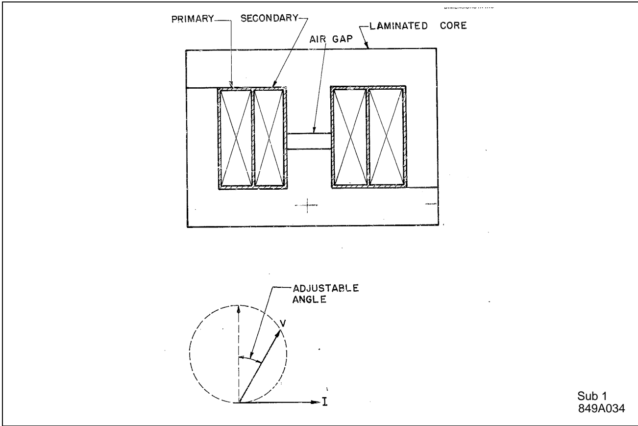
Figure 2: Compensator Construction
