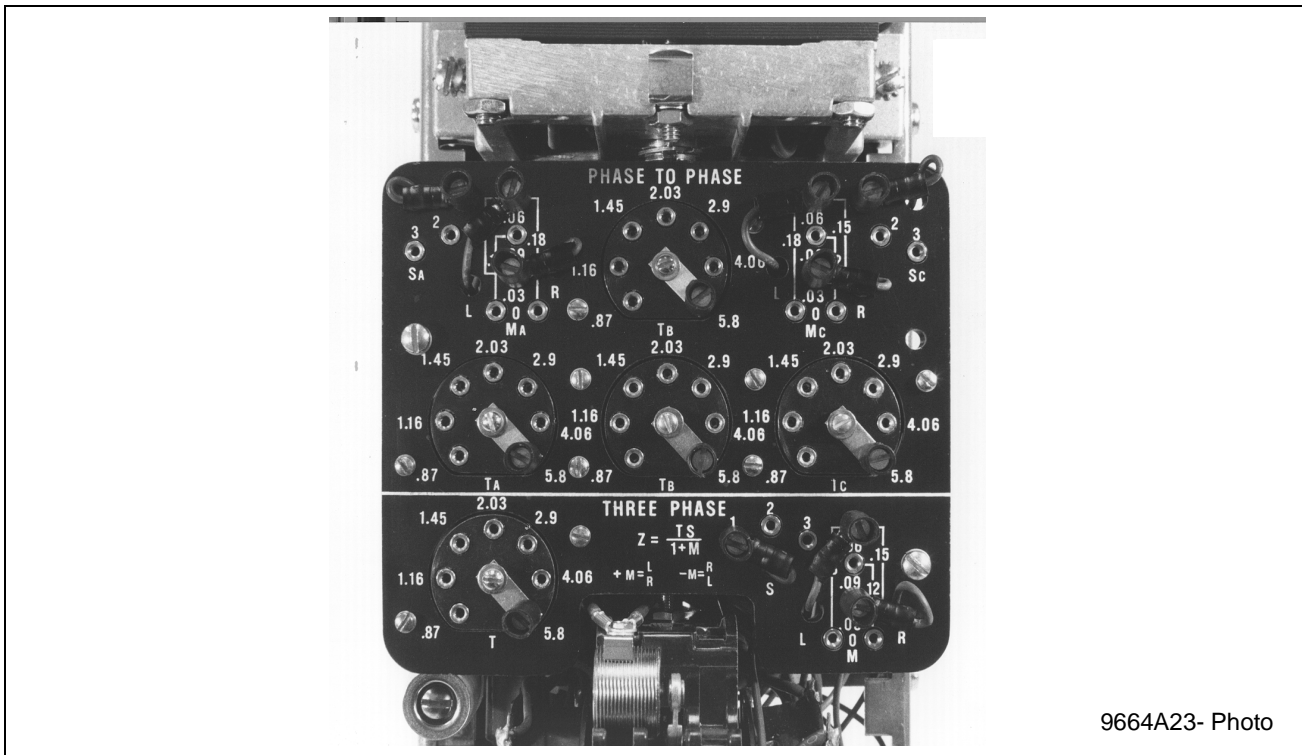
Figure 3: Typical Tap Plate
