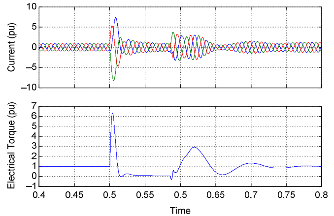
Fig. 4. Low-penetration three-phase fault
