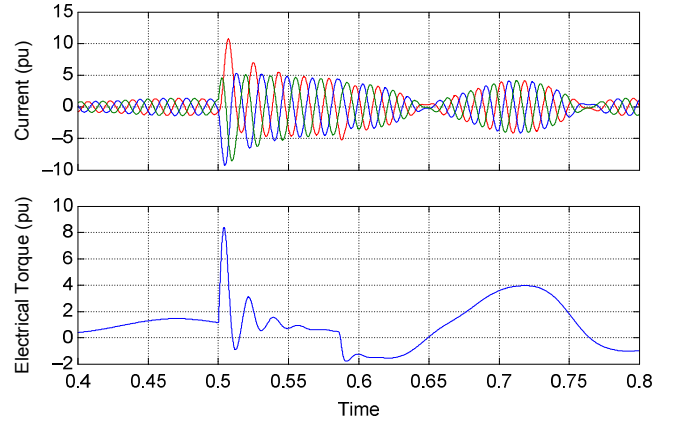
Fig. 6. High-penetration three-phase fault
