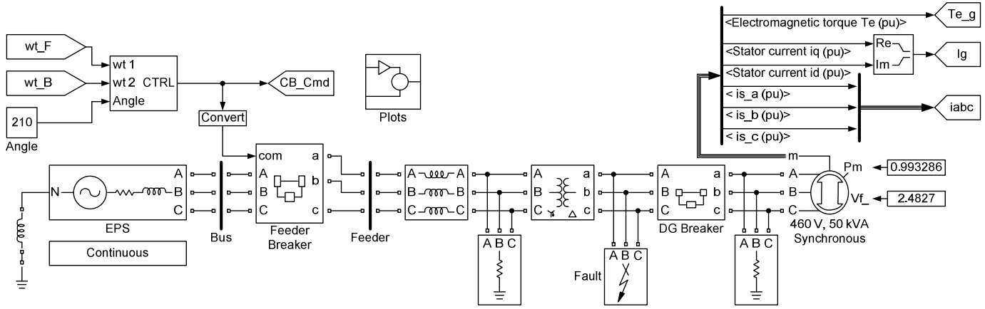
Fig. 3. Low-penetration model
