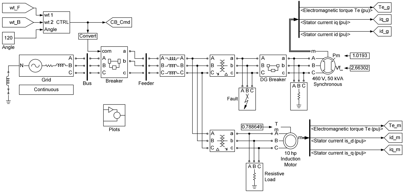
Fig. 8. Low-penetration model with a motor load
