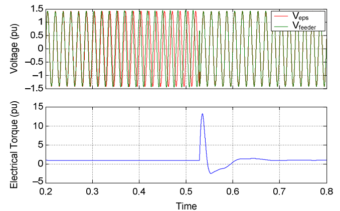
Fig. 5. Low-penetration reclose at 120 degrees
