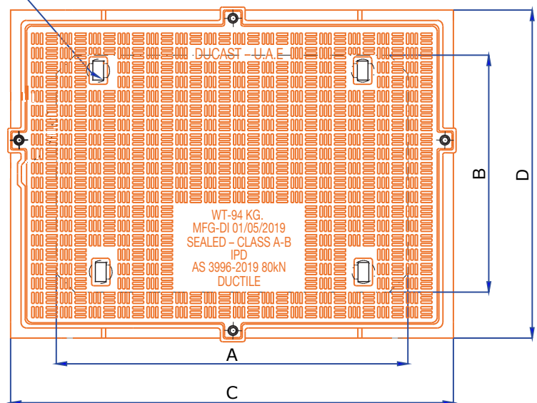
PLAN OF COVER & FRAME
