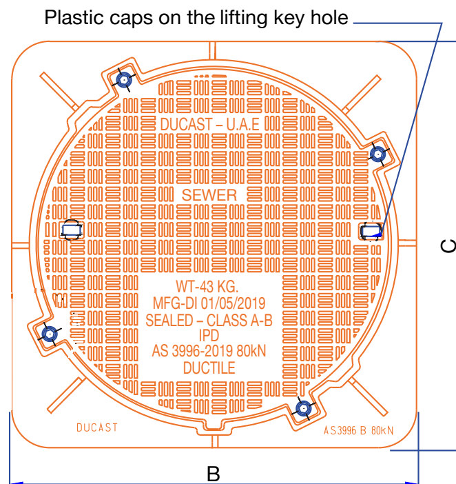
PLAN
