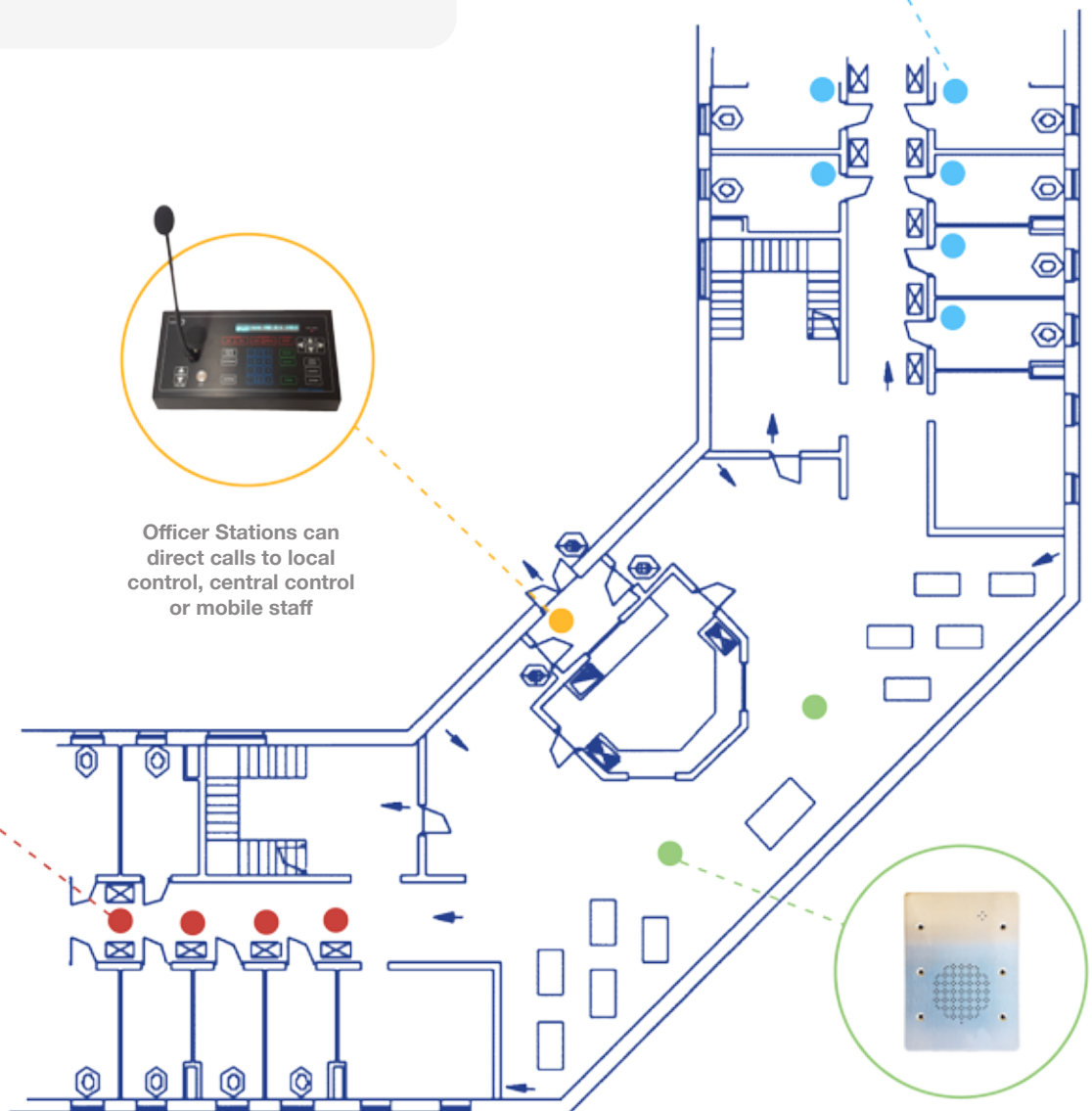
Ceiling monitored PA speakers are installed in common areas
